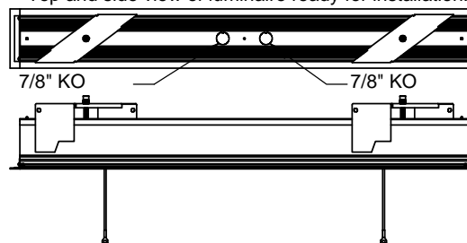
Top and side view of luminaire ready for installation.
