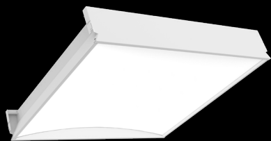
Concave Lens
