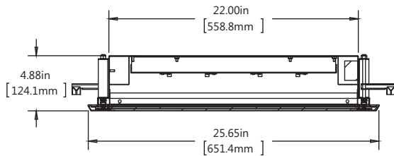
CROSS SECTION
